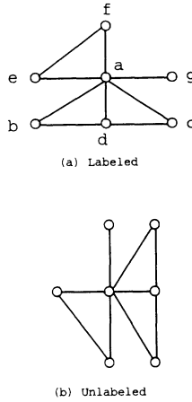
FIGURE 8. Labeled graph and underlying unlabeled graph.
