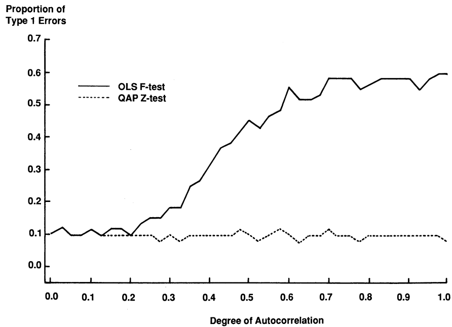
Fig. 1. Plot of Type 1 error rates of significance tests for simple regression coefficients.
