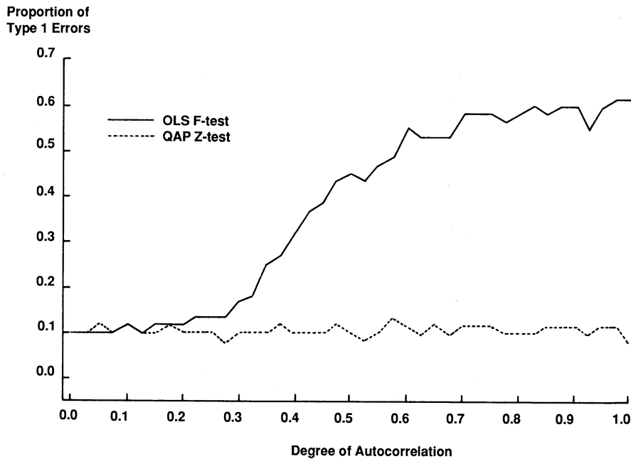
Fig. 2. Plot of Type 1 error rates of significance tests for multiple regression coefficients.
